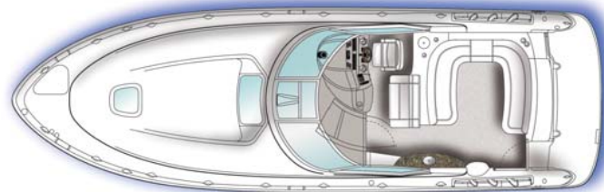
Cockpit Layout
